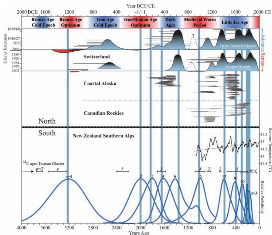
Fig. 3. The timing of Holocene glacier fluctuations near Mount Cook in New Zealand's Southern Alps ( bottom ), together with published ^{14}\text{C} ages on soils buried by Mount Cook glacier expansion events (11) over the past 4000 years, and a tree ring reconstruction of austral summer temperature in New Zealand over the past 1100 years (21), compared with glacier fluctuations in the Northern Hemisphere ( top ). The probability plots at the bottom are summary curves of all individual ^{10}\text{Be} boulder ages from each moraine dated in New Zealand. The blue bars show the arithmetic means of the moraine age (fig. S1 and table S3). The ^{10}\text{Be} ages are from Mueller Glacier moraines, except for the 1650-year moraine (Tasman Glacier) and 1370- and 1020-year moraines (Hooker Glacier). Note that we have identified a moraine corresponding to each ^{14}\text{C} soil age except for the 2300-year soil. The top graph shows fluctuations of two index glaciers in the Swiss Alps, the Great Aletsch Glacier and the Gorner Glacier, reconstructed from historical accounts and tree ring and radiocarbon data from fossil wood by (30). The middle graph shows the glacier advances in coastal Alaska (31) and the Canadian Rockies (32). These northern records feature high-precision glacier chronologies derived primarily from dendrochronology. Each bar shows the length of a tree ring record. The right end of each bar represents a glacier kill date.
